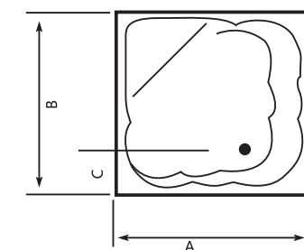
ST-110 Acrylic Shower tray
